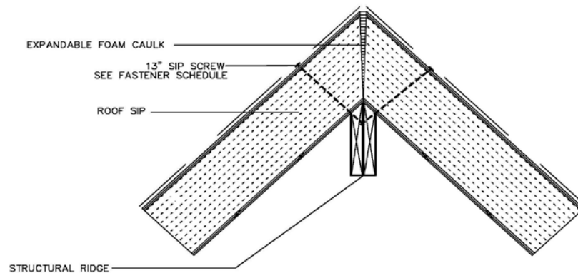
RIDGE DETAIL
